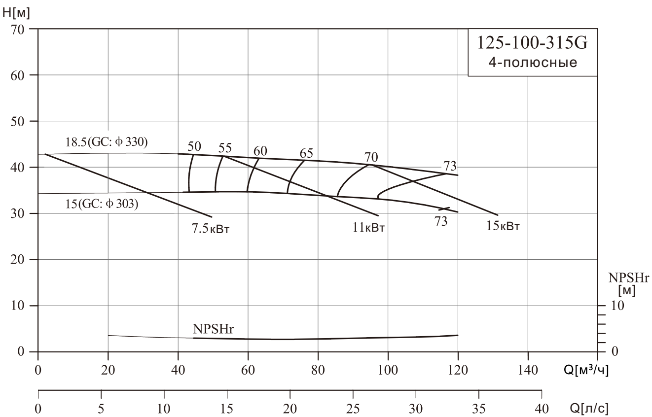
NIS125-100-315G/125-100-400G
