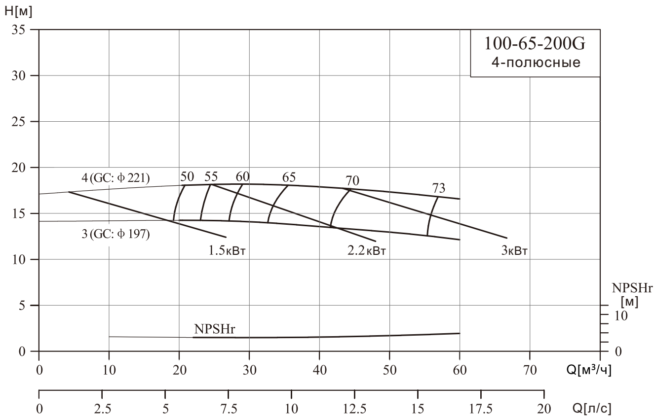
NIS100-65-200G/100-65-250G
