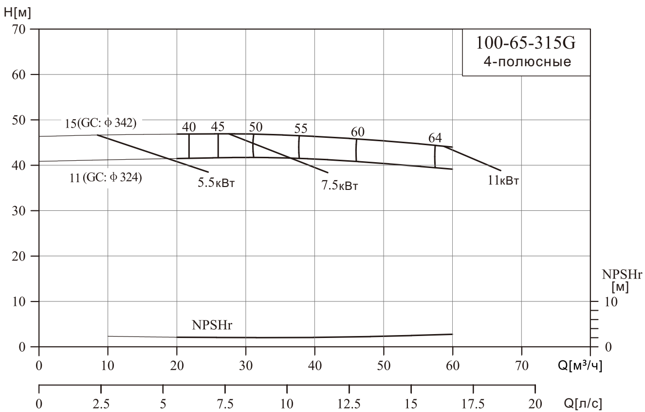
NIS100-65-315G/100-80-160G
