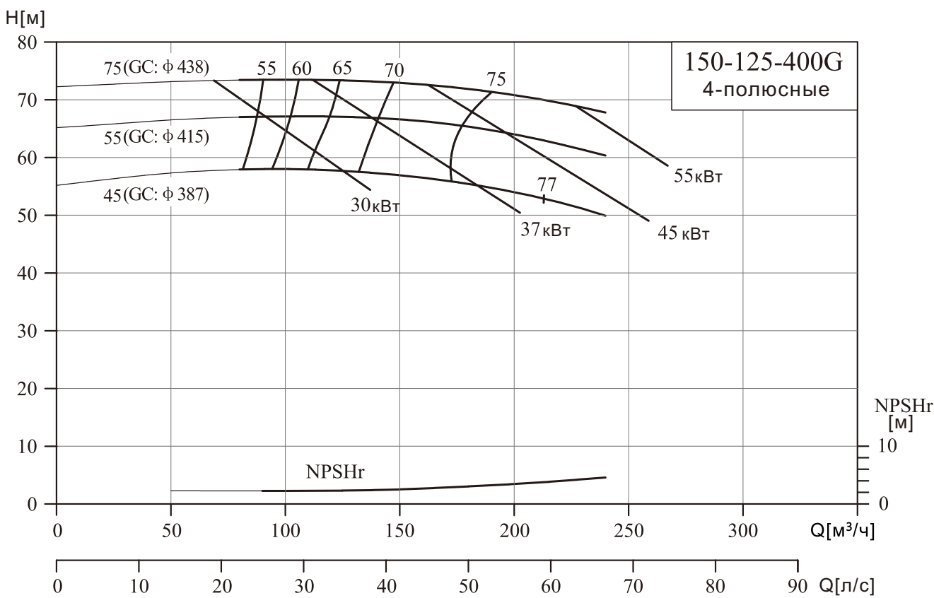
NIS150-125-400G/200-150-250(Q)
