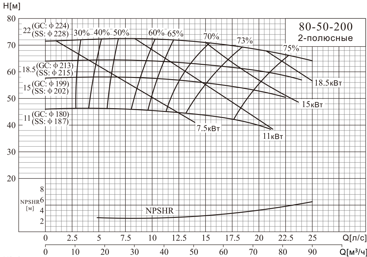
NISO,NIS,NISF 80-50-200/80-50-250
