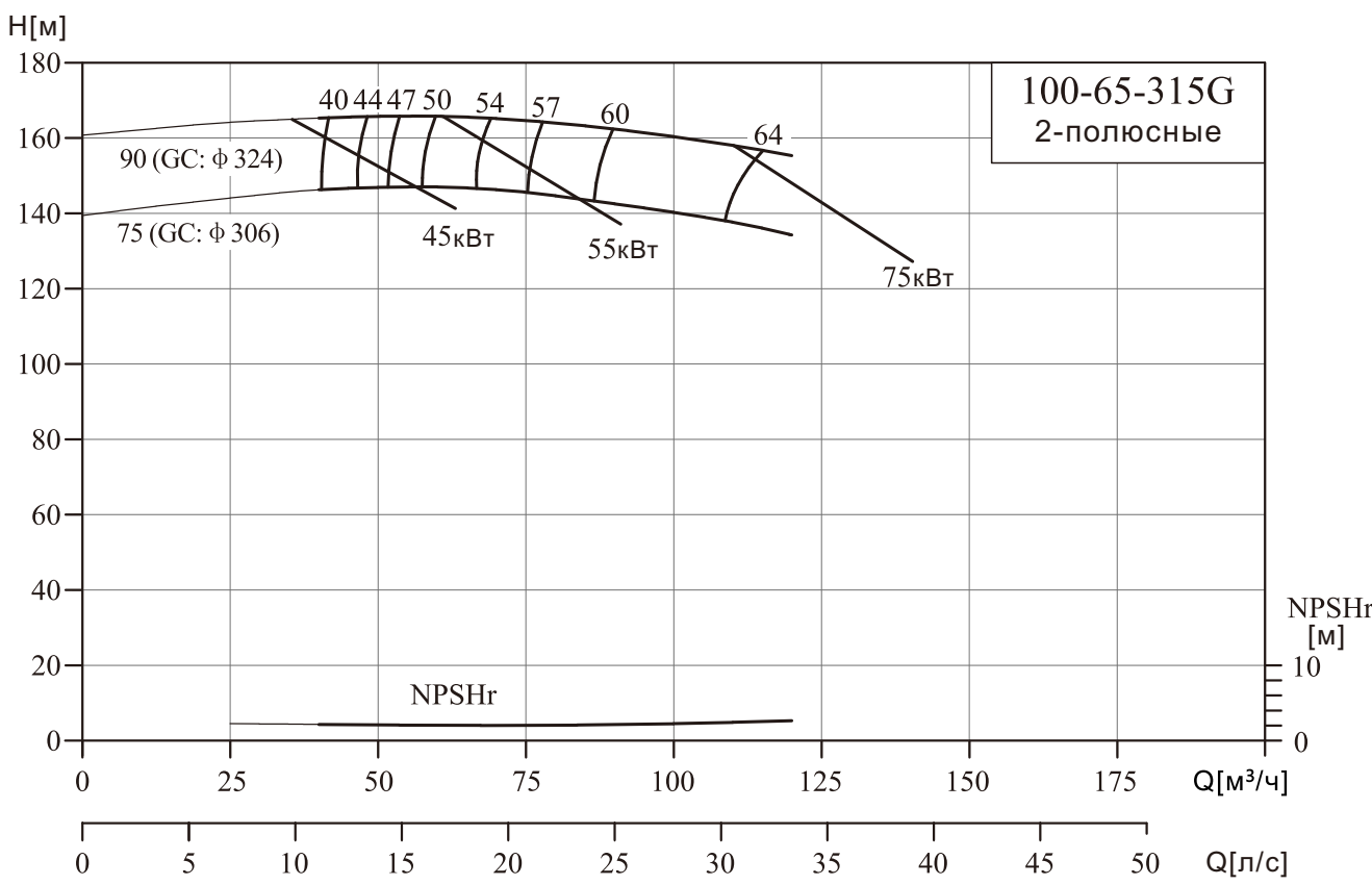
NIS100-65-315G/100-80-160G
