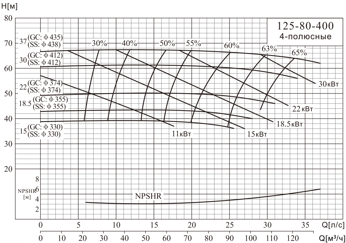
NISO,NIS,NISF 125-80-400/125-100-400
