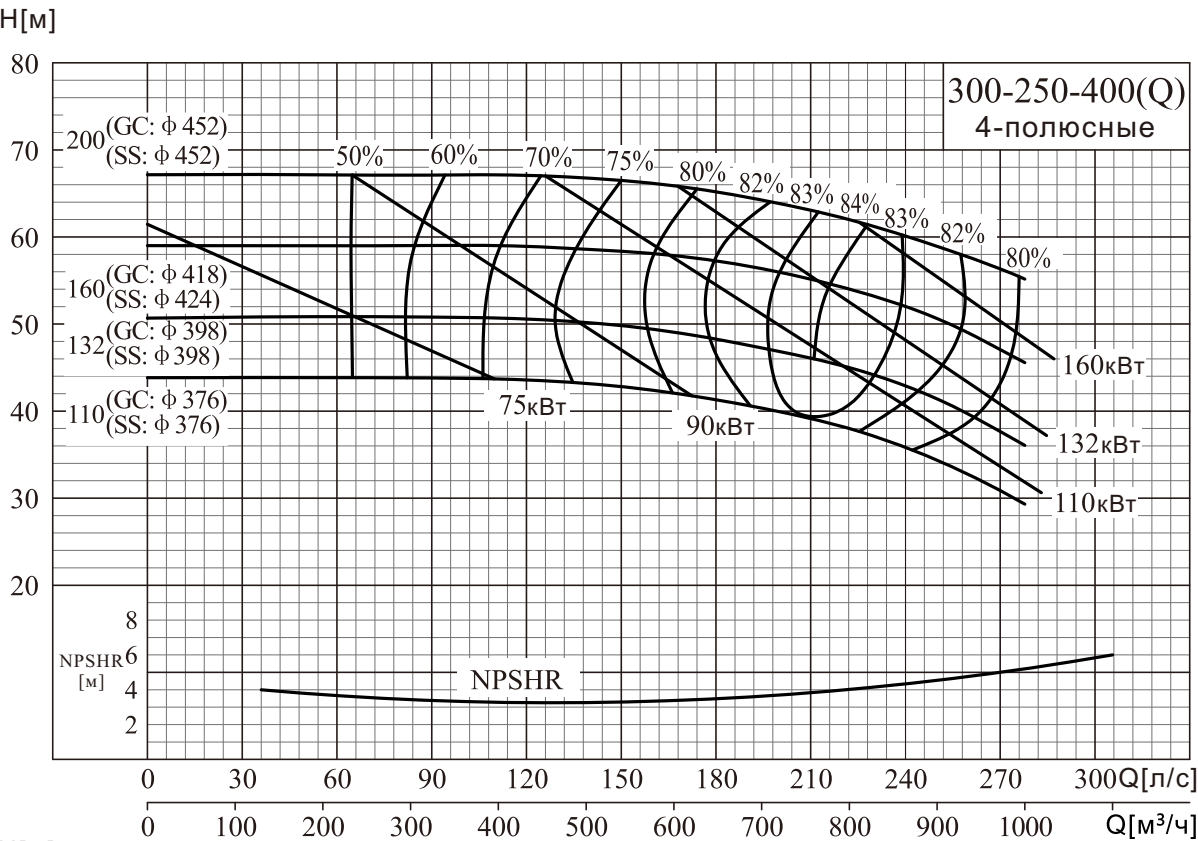
NISO,NIS,NISF 300–250–400(Q)/300–250–315
