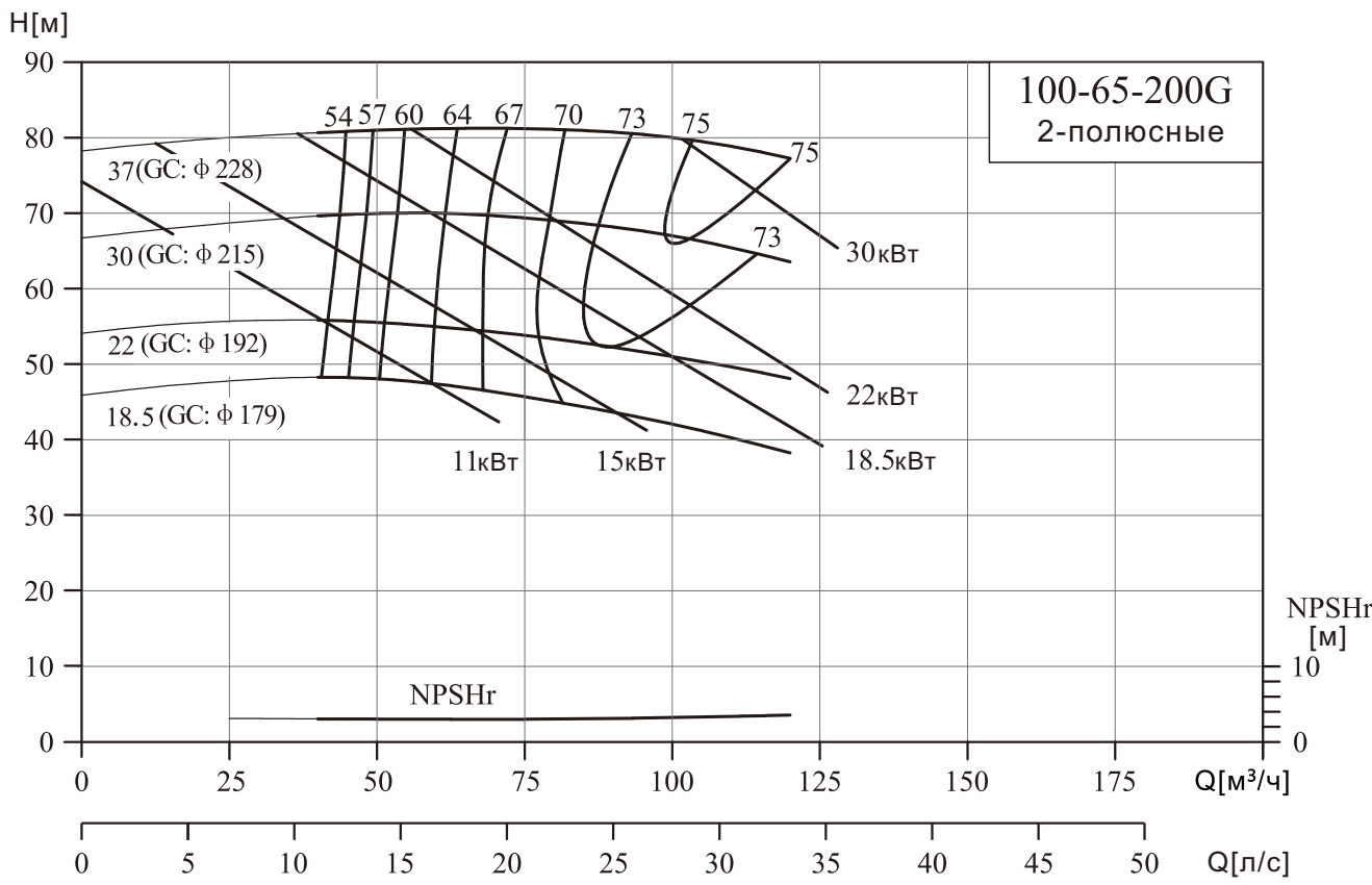
NIS100-65-200G/100-65-250G
