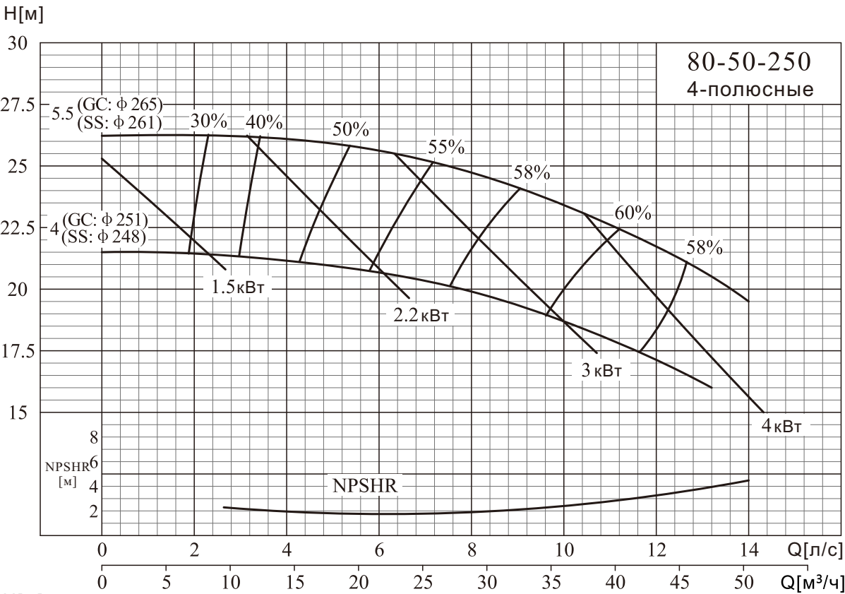
NISO,NIS,NISF 80-50-250/80-50-315
