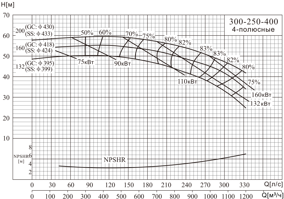
NISO,NIS,NISF 300–250–400
