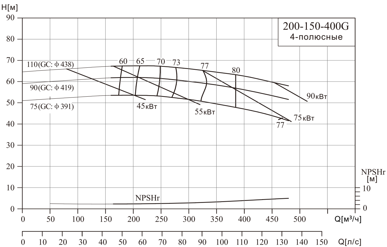
NIS200-150-400G
