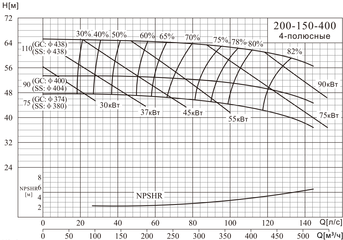
NISO,NIS,NISF 200–150–400/250–200–315
