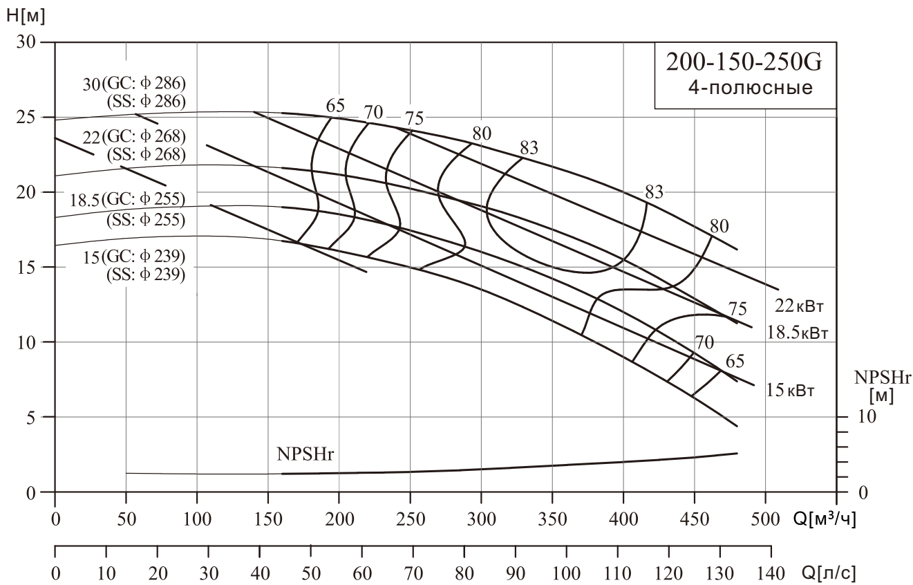
NIS200-150-250G/200-150-315G
