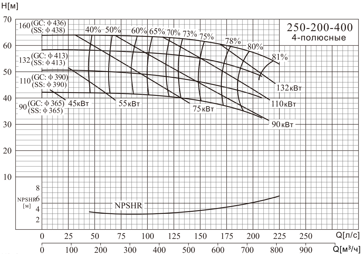
NISO,NIS,NISF 250–200–400/300–250–315(Q)
