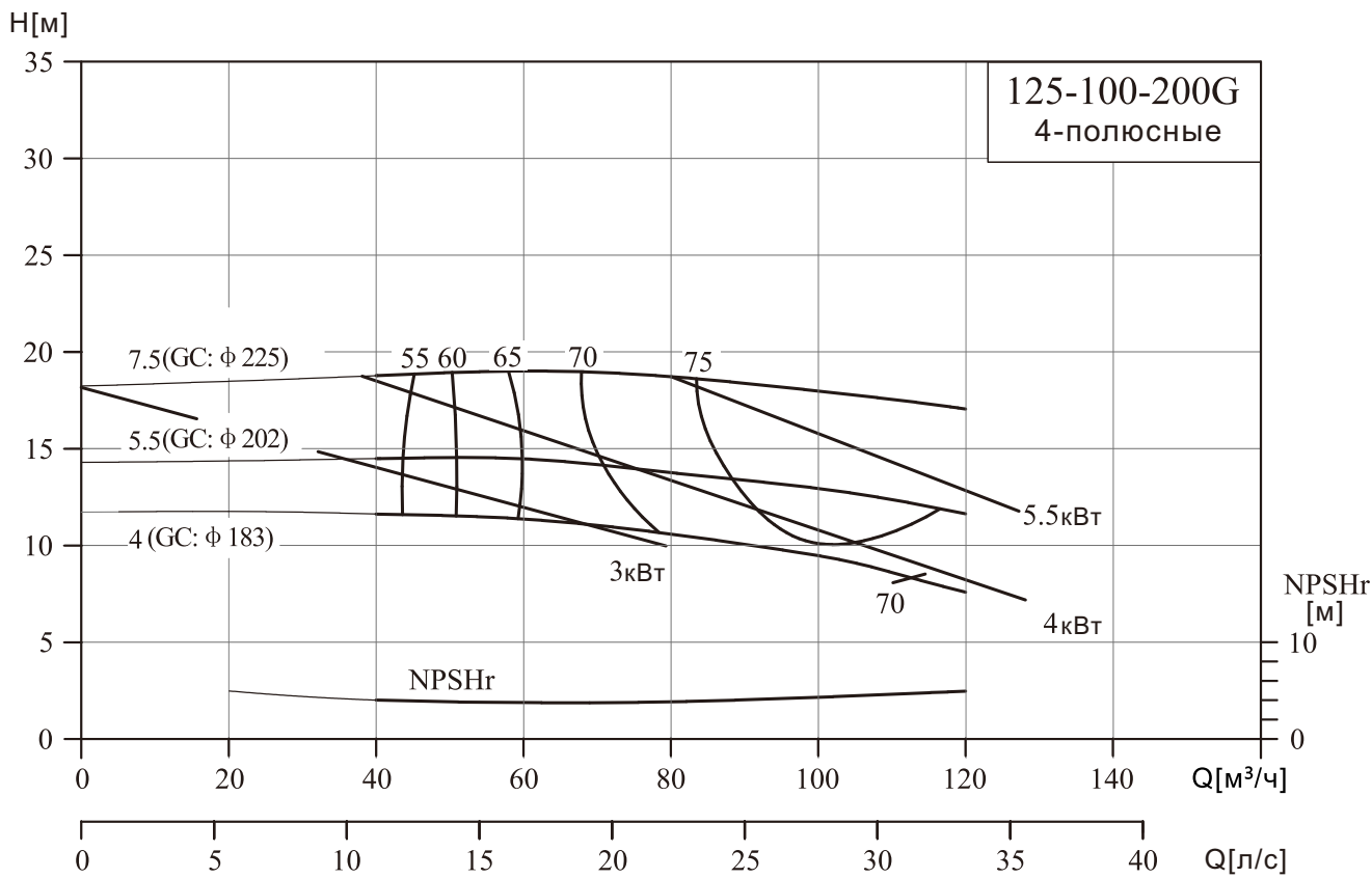
NIS125-100-200G/125-100-250G
